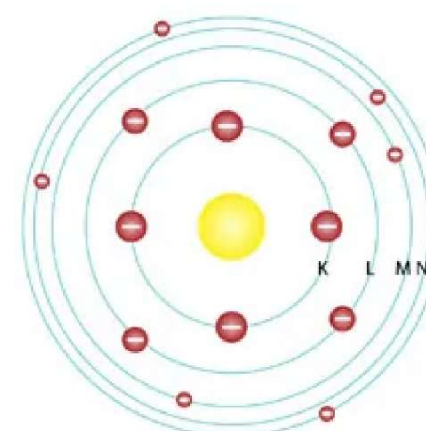
NIELS BOHR, 1913
