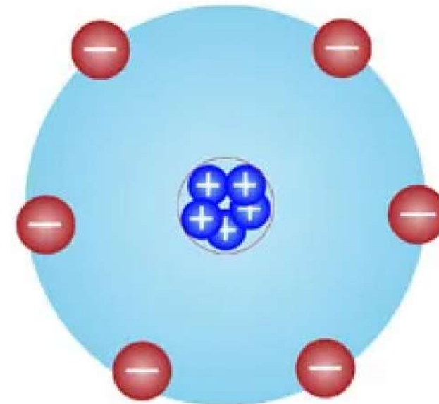
ERNEST RUTHERFORD, 1911
