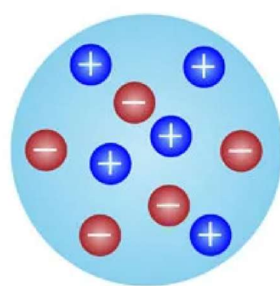
JJ THOMSON, 1904
