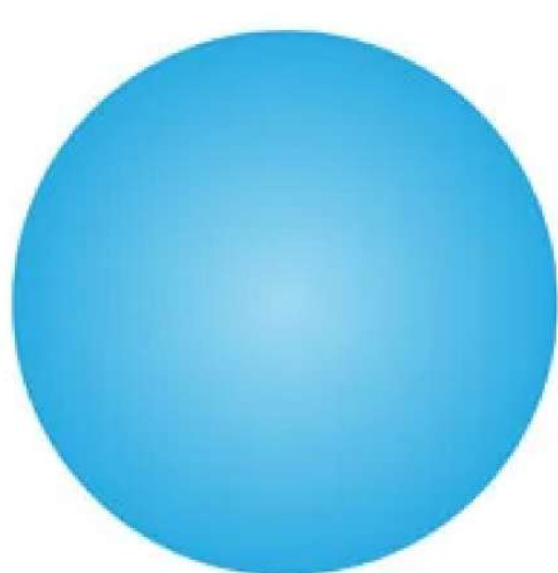
JOHN DALTON, 1803
